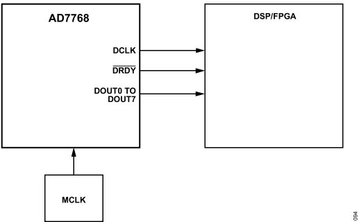
Figure 107. Data Interface: Standard Conversion Operation, AD7768 = Master, DSP/FPGA = Slave
