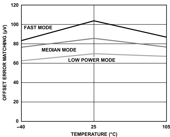
Figure 50. Channel Offset Error Matching
