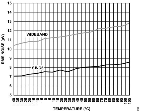
Figure 29. RMS Noise vs. Temperature, Fast Mode
