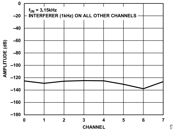
Figure 33. Crosstalk
