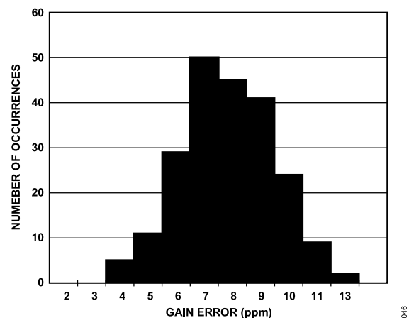
Figure 52. Channel to Channel Gain Error Matching
