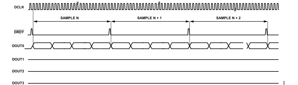
Figure 105. AD7768-4 FORMAT0 = 1: Channel 0 to Channel 3 Output on DOUT0 Only, Maximum Data Rate
