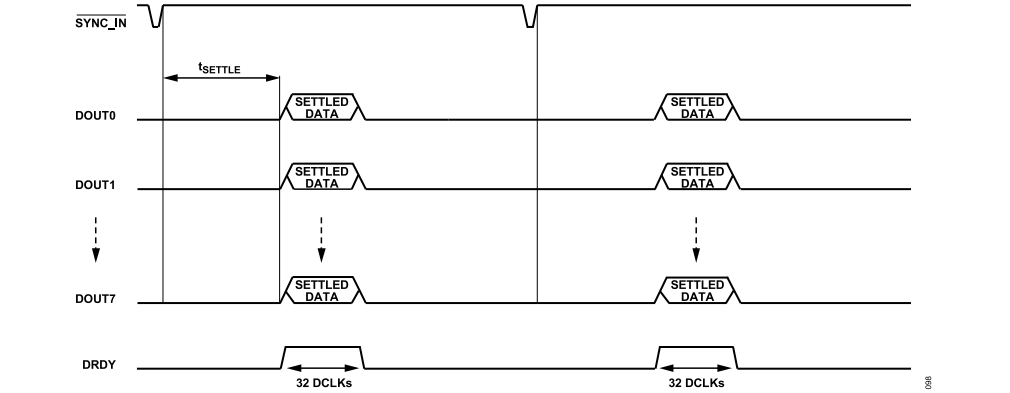
Figure 108. AD7768 One Shot Mode
